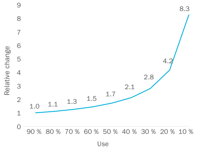
47 Relative change in LCOE with falling use of nuclear
