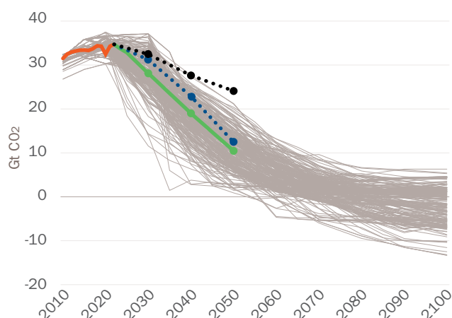
34 Emissions in the Scenarios vs IPCC 2°C (left) and IPCC 1.5°C (right) 88
