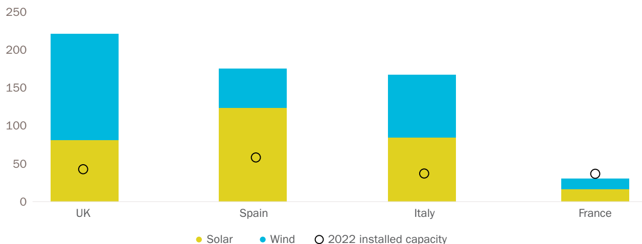
32 Wind and solar projects waiting to be connected to the grid (GW) 80
